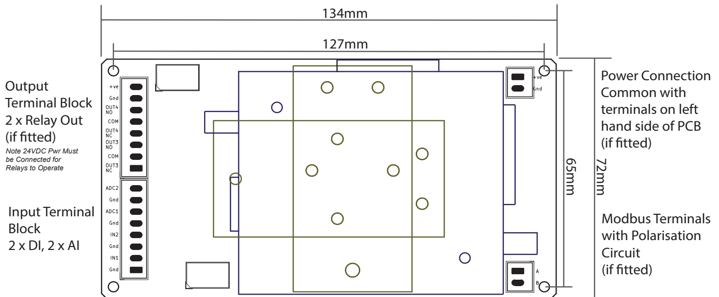
DIN Clip Mounting Positions with Mounting Holes (dia 3.3mm) shown
